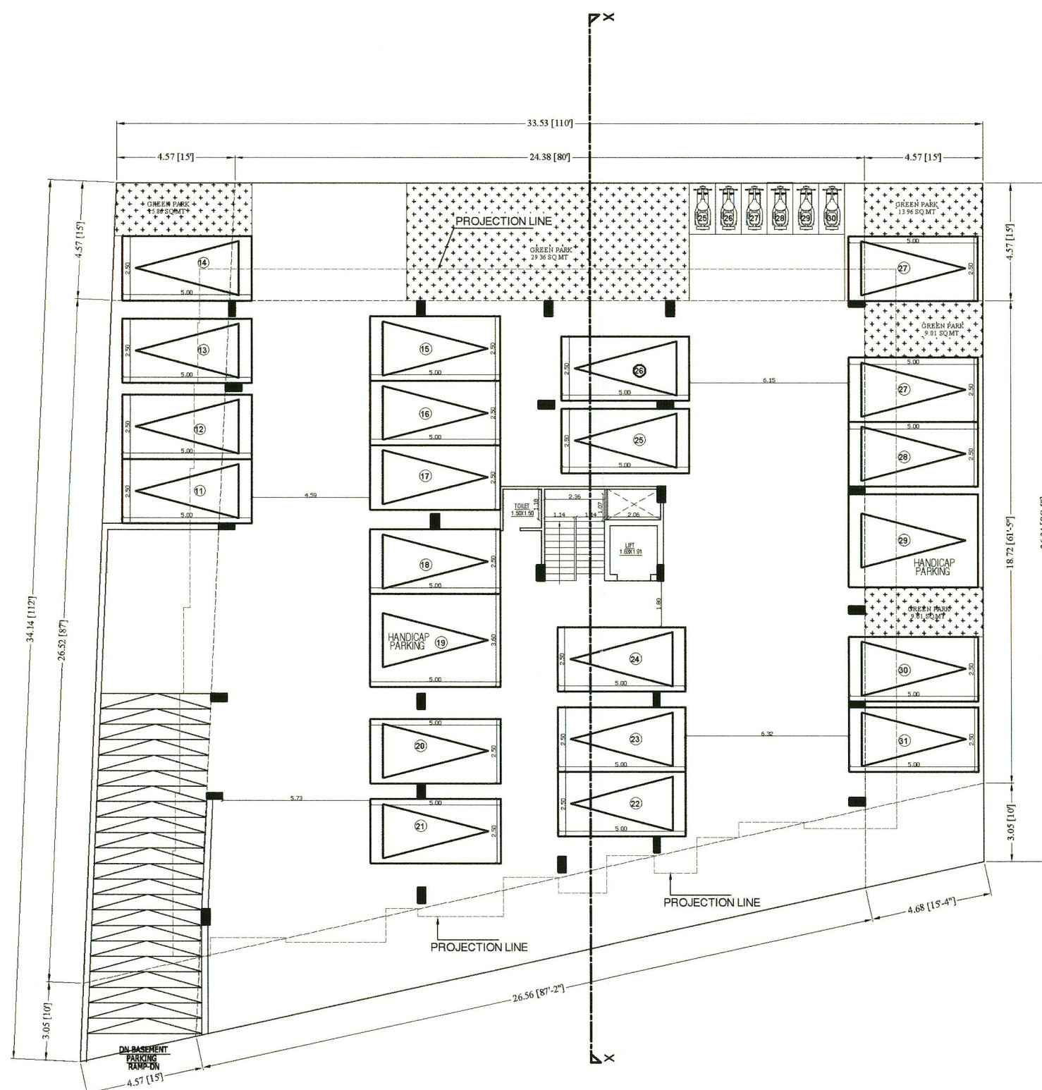
STILET FLOOR PLAN
