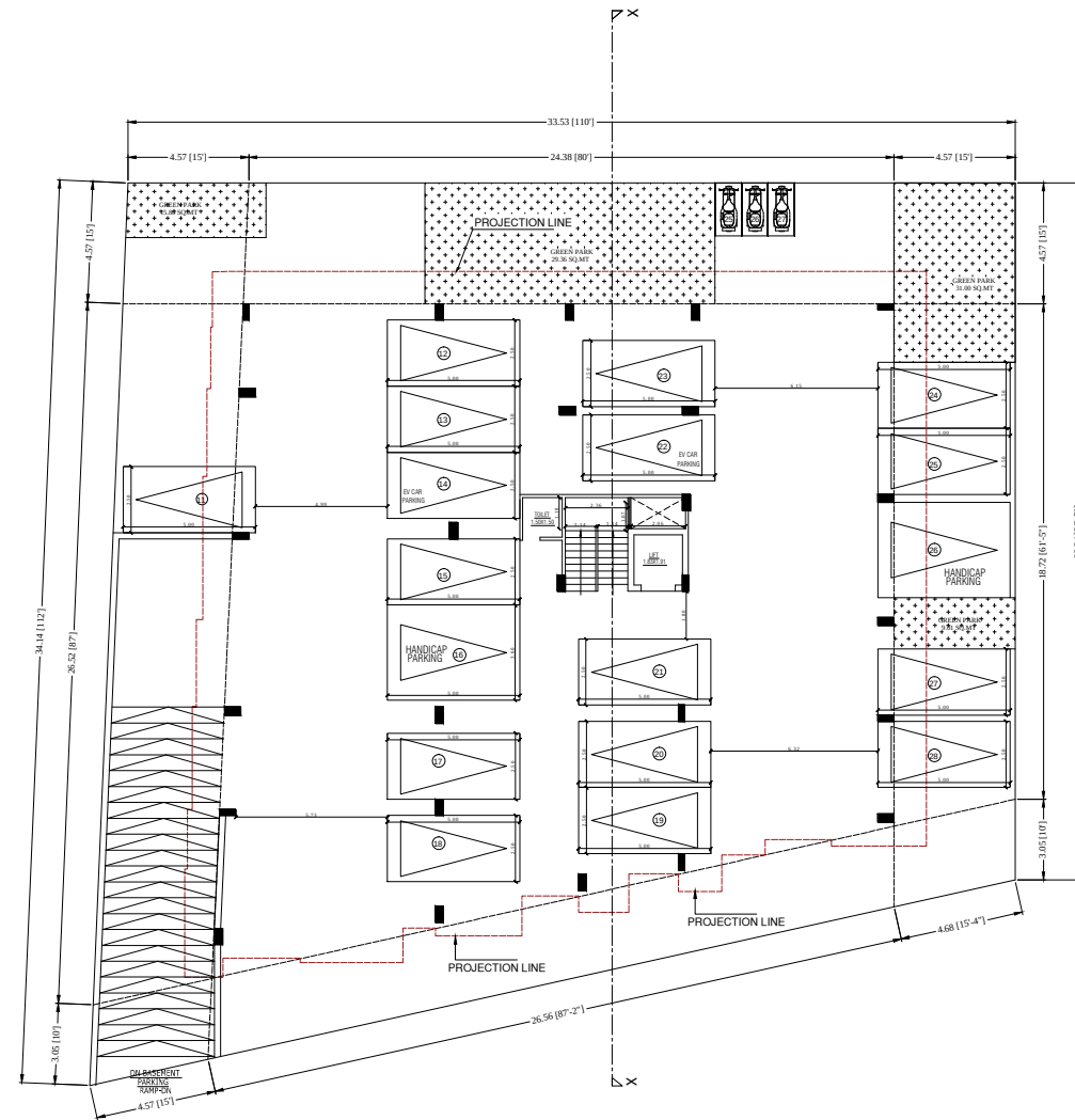
STILET FLOOR PLAN
